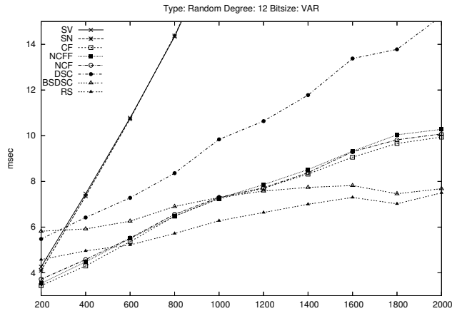
Figure 3. [3darr] polynomials
